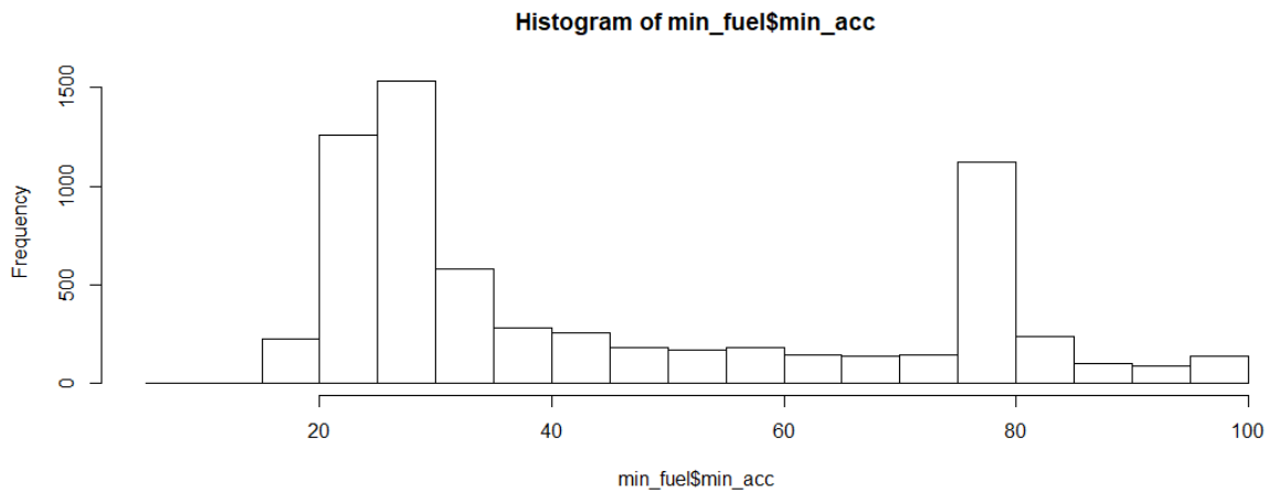
fig. 1 Histogram of starting battery level when transaction is ended at a charging station
