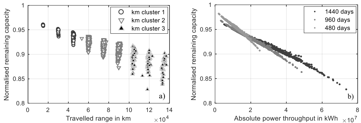
Figure 6: Dependency of battery aging on mileage a) and energy throughput b)
