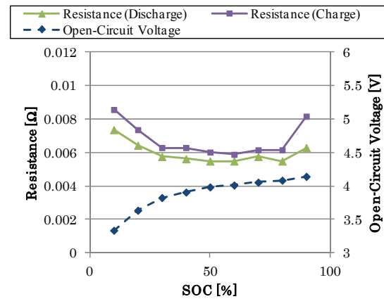
Figure 2: Characteristics of Internal Resistance and Open-circuit Voltage of the Lithium-ion Battery (Single Cell)
