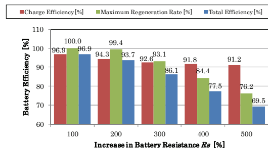
Figure 8: Charge Efficiency and Permissible Recovery Rate of Regenerated Power per Internal Resistance Increase
