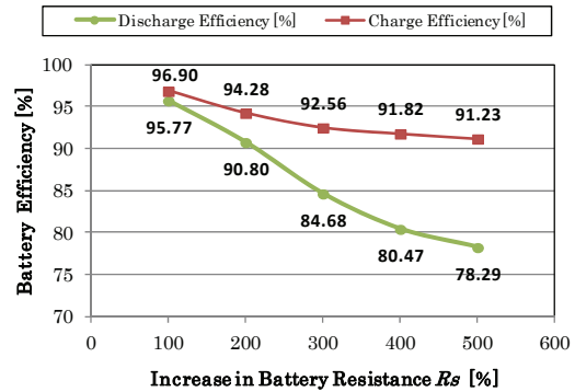
Figure 6: Charge and Discharge Efficiency when Internal Resistance Increases
