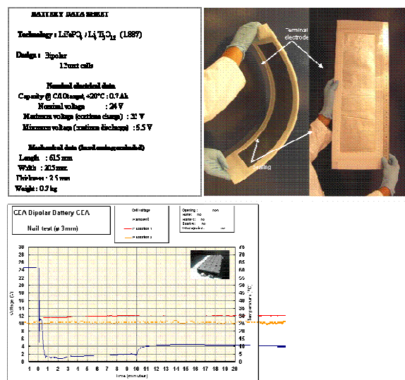
Figure 2: CEA 15 Wh Li ion bipolar cell data sheet and photography.
