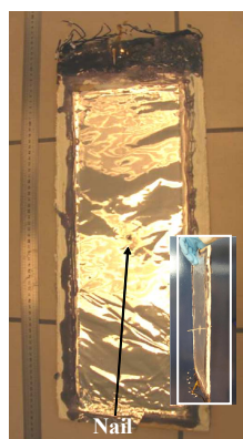
Figure 6: Safety test. Li ion bipolar cell photography after perpendicular nail penetration.
