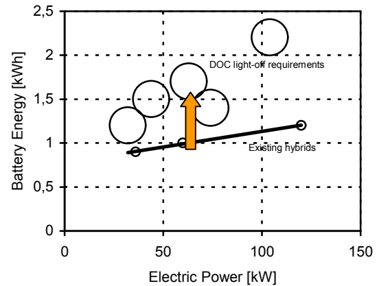
Figure 15: Increased requirements due to DOC light-off control. Battery energy based on estimated usable energy assuming 50% SOC window
