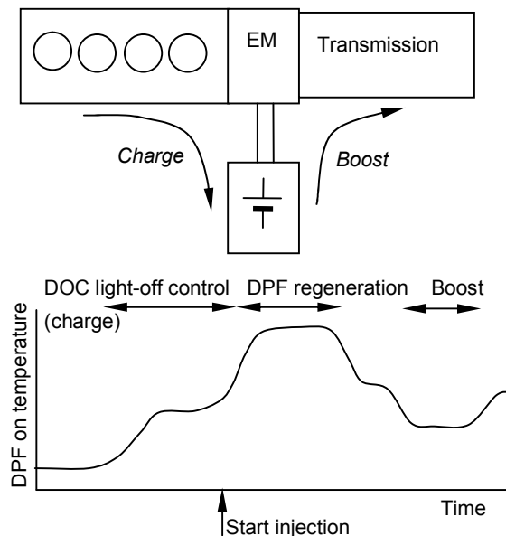
Figure 6: Principles of hybrid-assisted DPF regeneration
