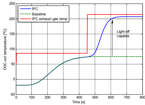
Figure 12: Exhaust and DOC temperature, regeneration from idle @ -20^{\circ}\text{C} . Control is started at 450s.
