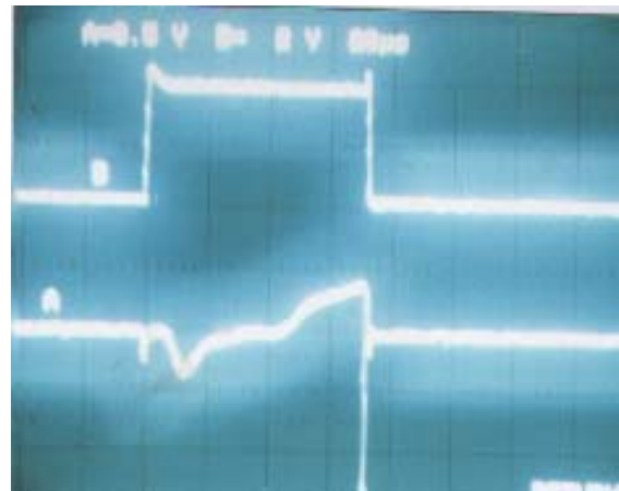
Fig (3) BJT base to emitter voltage and emitter current.
