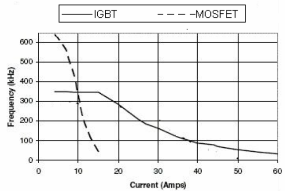
Fig 2 Usable frequency vs. current
