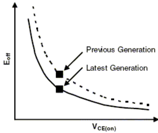
Fig. 1 Turn-Off Energy vs. V_{CE(on)}
