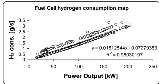
Figure 8: FC experimental data
