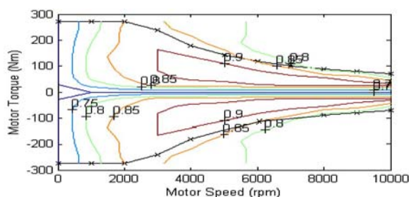
Figure 10: Westinghouse 75 kW from ADVISOR
