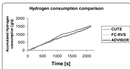
Figure 11: Comparison between experimental (CUTE), ADVISOR and FC-RVS
