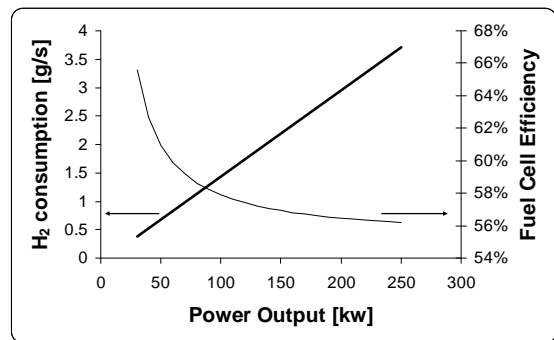
Figure 9: FC fuel consumption and efficiency used in the model
