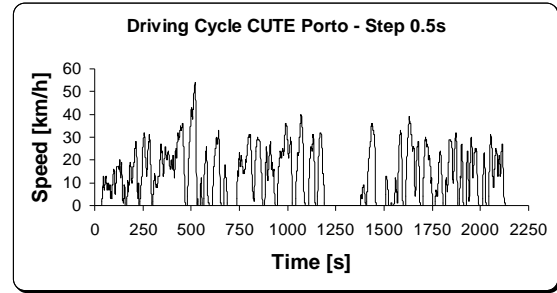
Figure 7: Driving cycle chart used in simulation
