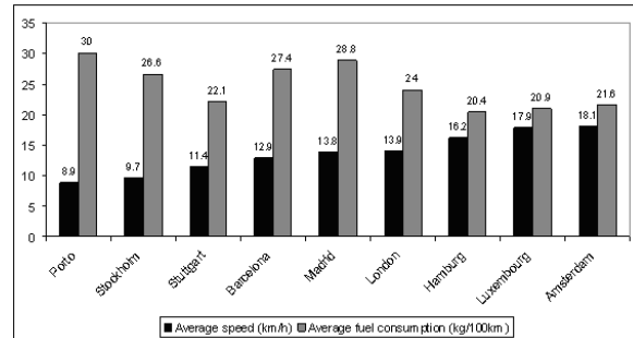
Figure 2: Comparison of average speed and fuel consumption in the cities of the CUTE project
