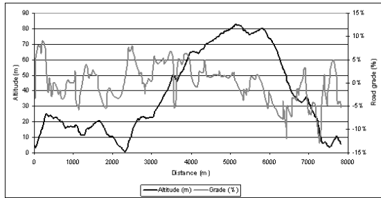
Figure 4: Topography and gradient profile
