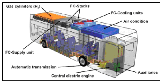
Figure 1: Layout of main elements
