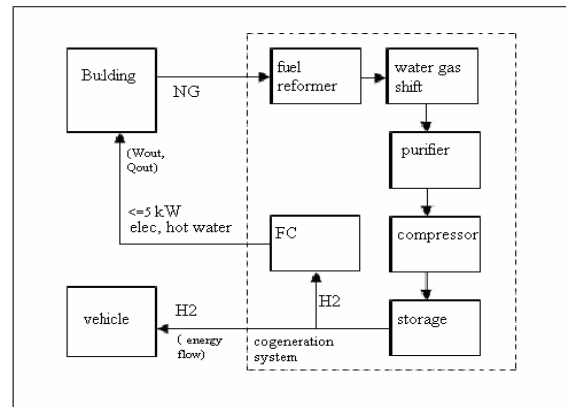
Figure 1 the schematic of a typical tri-generation system (source: [14])
