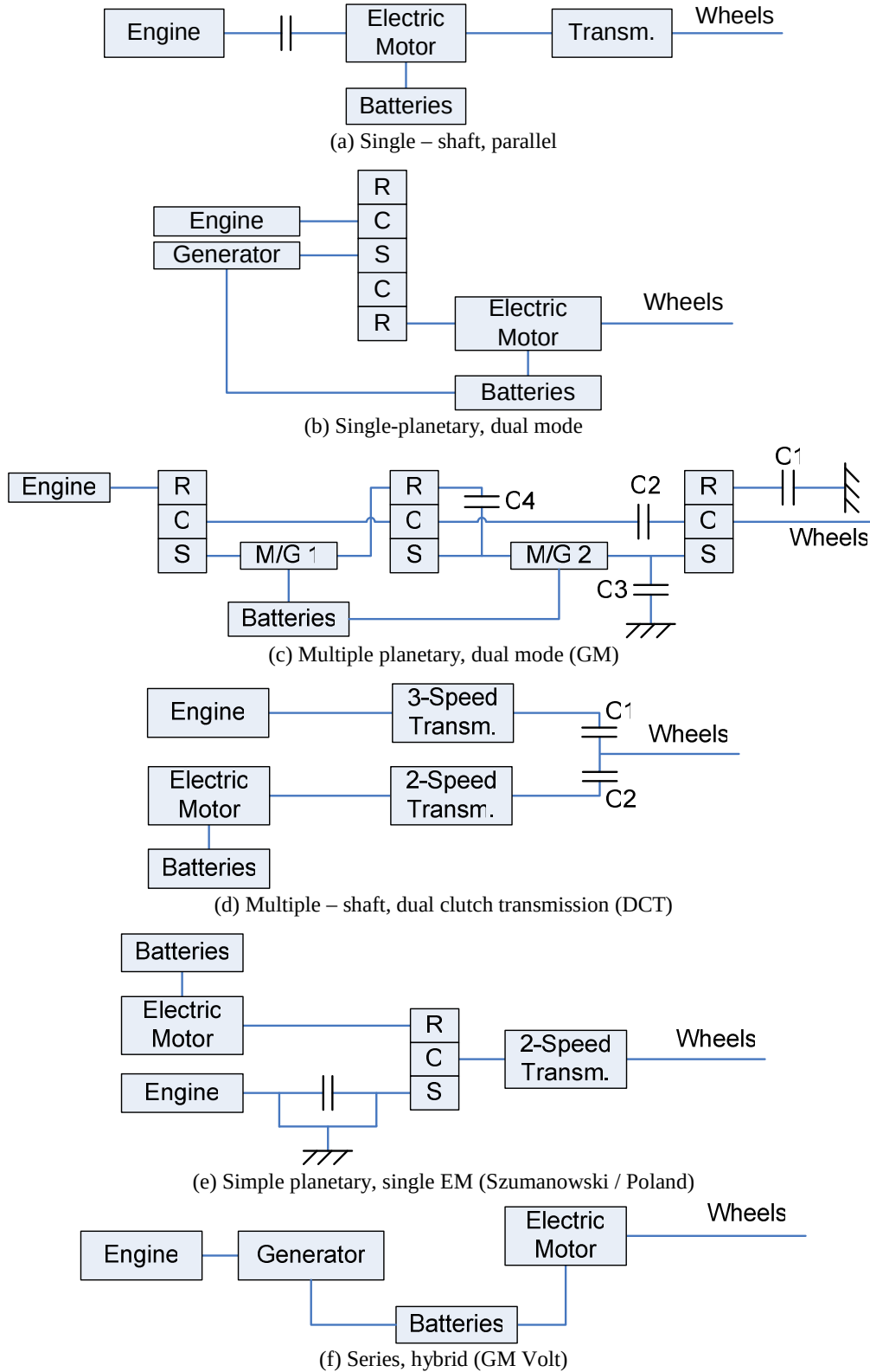
Figure 1 Schematics of various hybrid-electric powertrains
